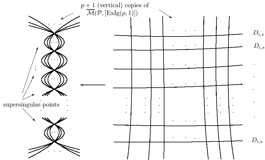
Figure 2: Katz-Mazur and stable fibers of X_i
