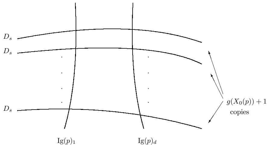
Figure 3: Special fiber of X_{ns}(p)_{\mathbb{F}_p}^{st}
