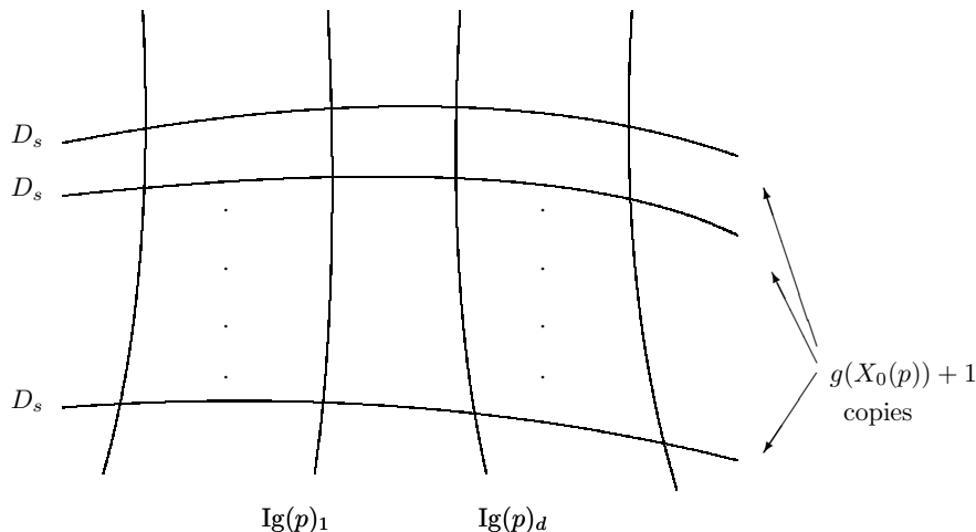
Figure 5: Special fiber of X_s(p)
