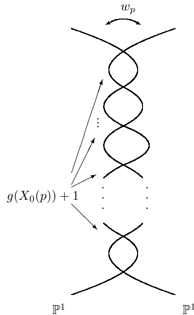
Figure 1: X_0(p)/\overline{\mathbb{F}}_p
