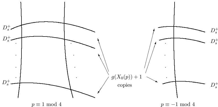
Figure 4: Special fiber on \overline{\mathbb{F}}_p of the semistable model X_{\text{ns}}^+(p) , depending on p \equiv \pm 1 \pmod 4
